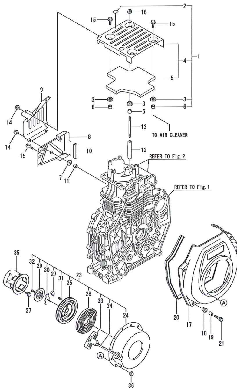
Fig.6. COOLING &amp; STARTING DEVICE
