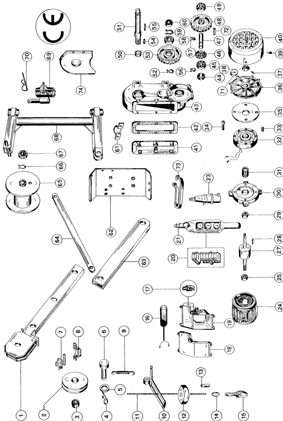
FIG. 12 — Despiece AY-300 GR
